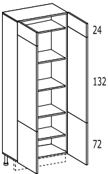
COLONNA 6 ante – 3 ripiani TALL UNIT 6 doors – 3 shelves
