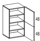
PENSILE DX O SX 2 ante – 2 ripiani RH/LH WALL UNIT 2 doors – 2 shelves
